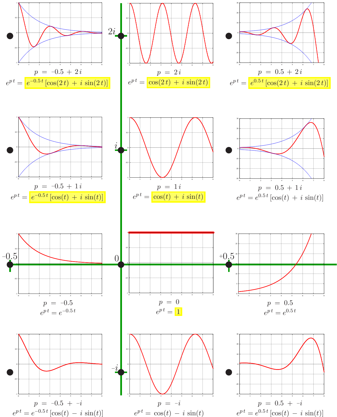
Figure 7.1: Pole location in the complex plane and behavior of e^{pt}
